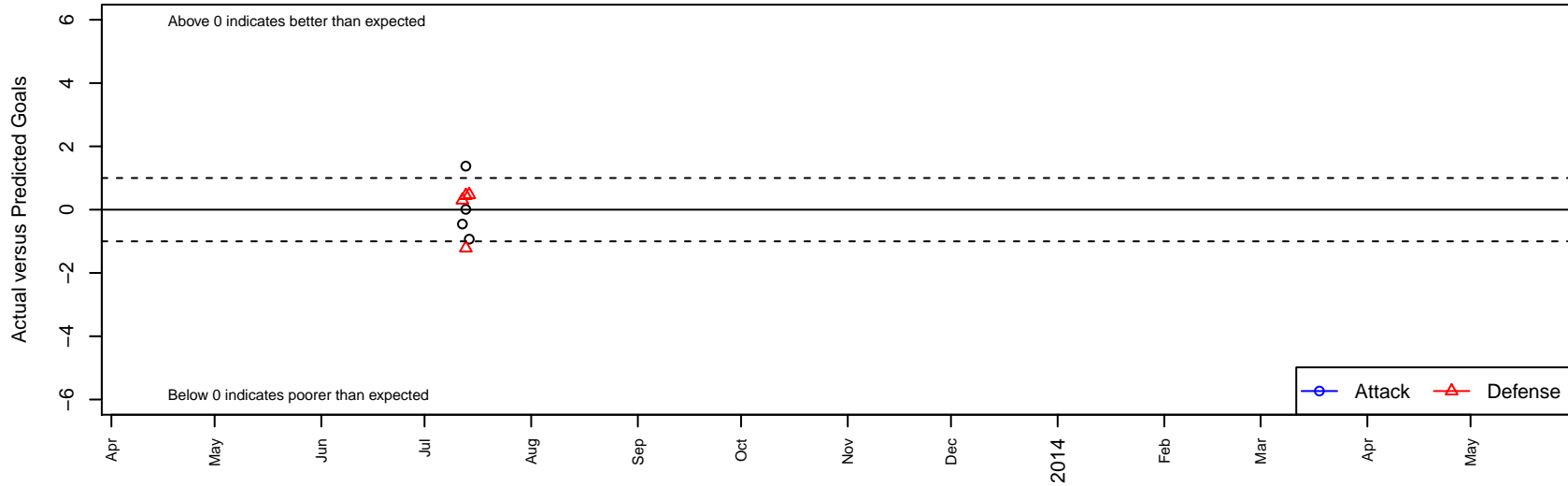
WFC Premier Red – Unk B99 Dots are actual minus expected GF (blue circles) and GA (red triangles). Blue line is smoothed change in attack strength. Red is smoothed change in defense strength.
